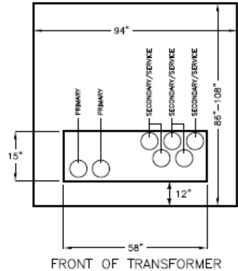
TOP VIEW OF PAD (DIMENSIONS MAY VARY)
